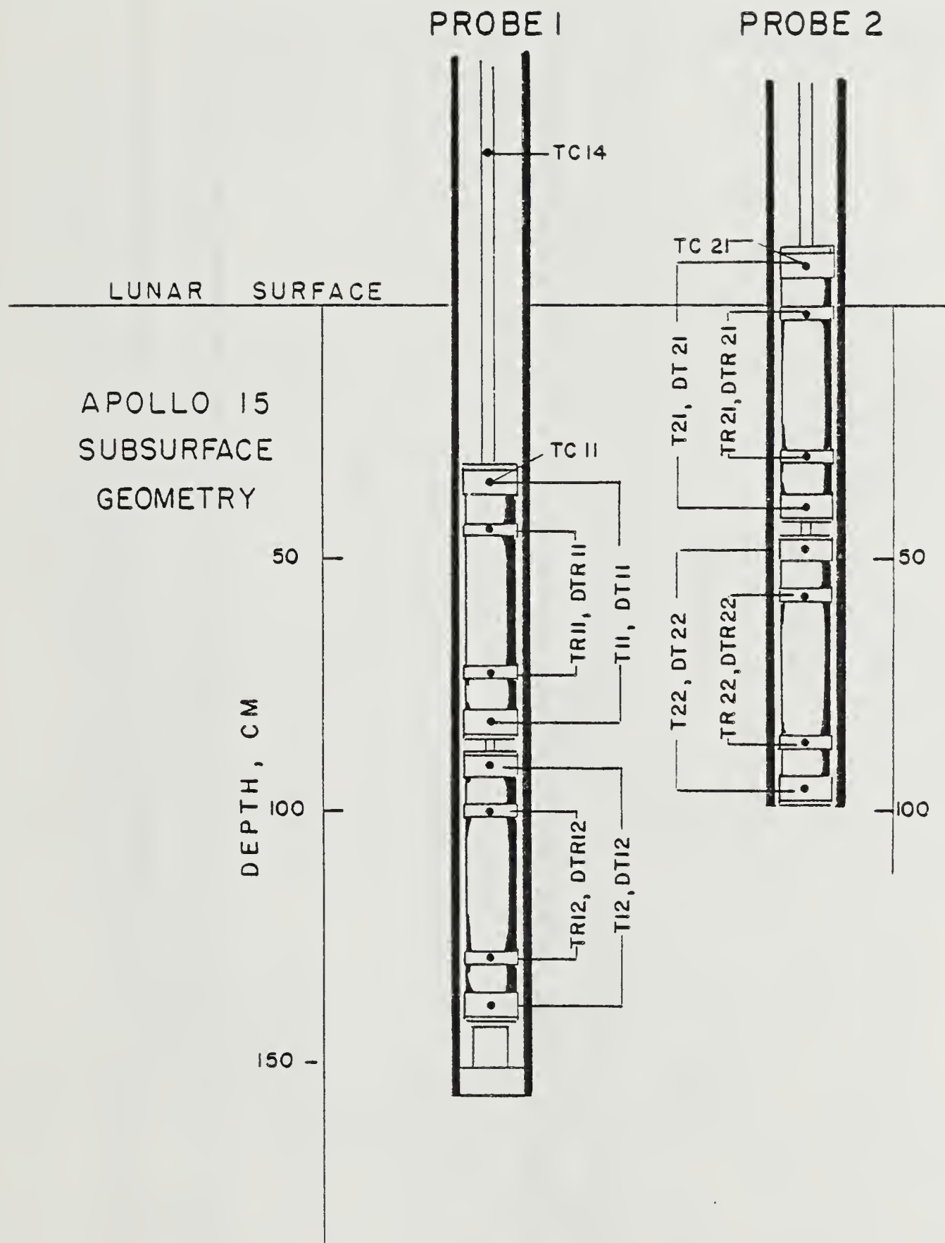
Configuration of the heat-flow probes in the lunar regolith. Additional details about the heat-flow instrumentation may be found in Langseth et al. (1974)
